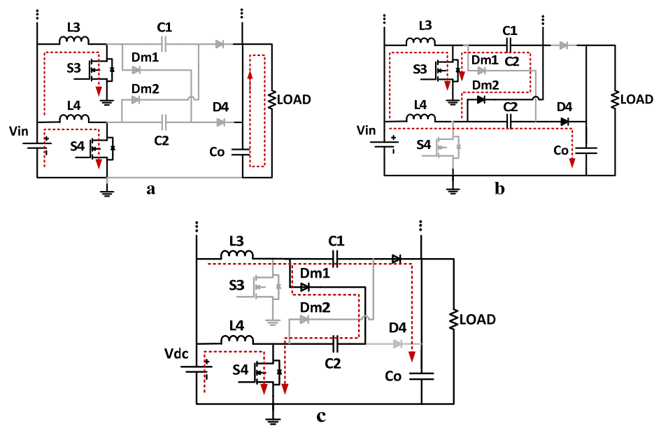
Fig. 2. Circuit topology and current paths in each operation interval (in the lower stage). (a) Interval 1&3, (b) Interval 2 (c) Interval 4
