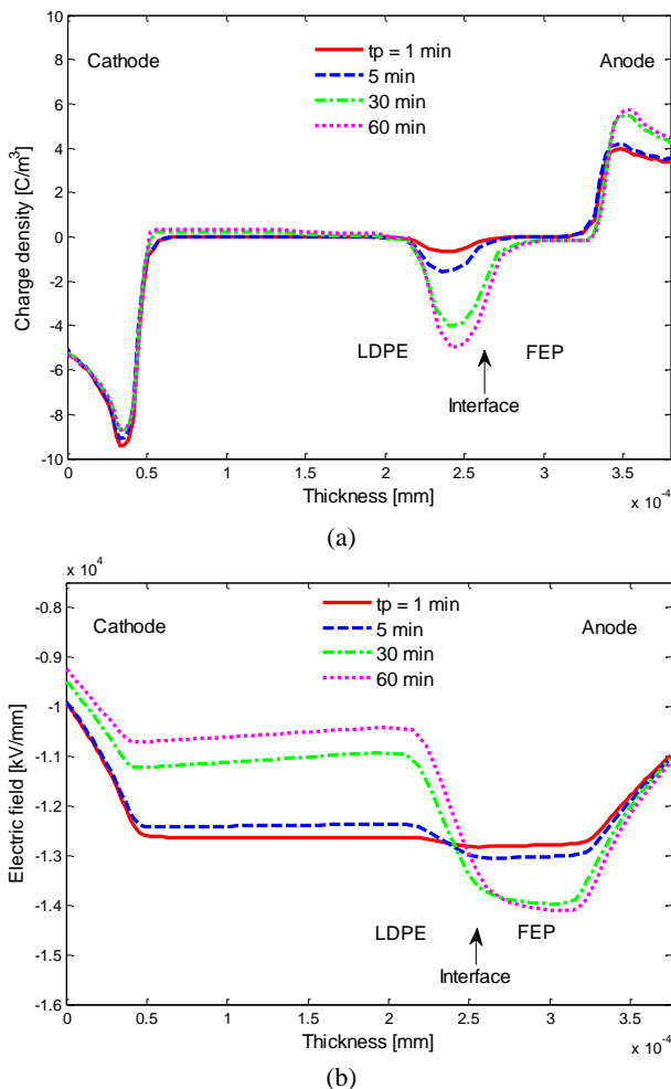
Fig. 4 Space charge and electric field distribution within a sandwich of LDPE-FEP with a negative charge at the dielectric/dielectric interface at T = 40^{\circ}\text{C} : (a) Charge profile during polarization, (b) Electric field during polarization ( T=40^{\circ}\text{C} ).
