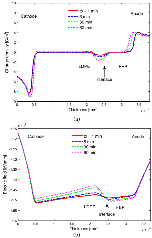
Fig. 3 Space charge and electric field distribution within a sandwich of LDPE-FEP with a negative charge at the dielectric interface at T = 20^\circ\text{C} : (a) Charge profile during polarization, (b) Electric field during polarization ( T=20^\circ\text{C} ).
