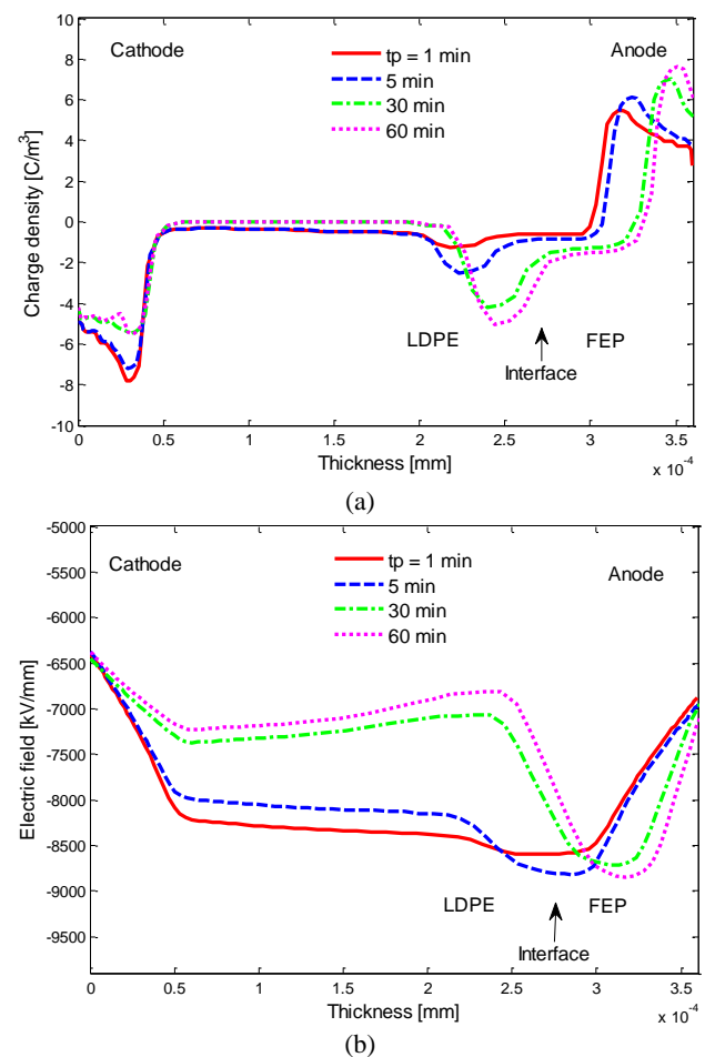
Fig. 5 Space charge and electric field distribution within a sandwich of LDPE-FEP with a negative charge at the dielectric/dielectric interface at T = 60^{\circ}\text{C} : (a) Charge profile during polarization, (b) Electric field during polarization ( T=60^{\circ}\text{C} ).
