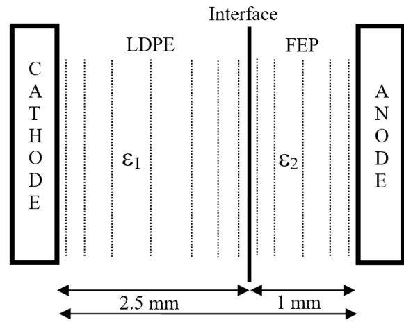
Fig. 2 Schematic representation of the LDPE-FEP system used for the simulation.
