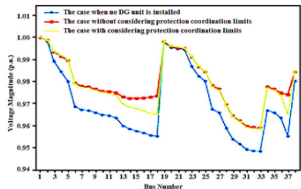
Fig. 4 Voltage profile for three different states.
