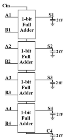
Fig. 8. 4-bit Full adder Test Circuit
