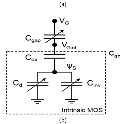
Fig. 1 a) Schematic of the RSG MOSFET b) Electrical equivalent circuit of the RSG-MOSFET showing the capacitive divider.
