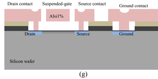
Fig. 8 Schematic of the fabrication process steps of a metallic RSG-MOSFET.
