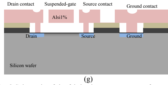
Fig. 8 Schematic of the fabrication process steps of a metallic RSG-MOSFET.
