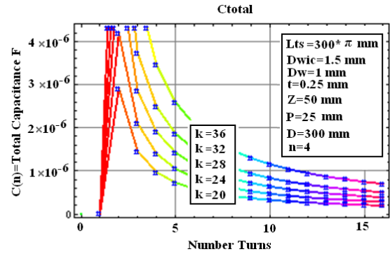
Fig. 18 Total capacitance of the HFCG for different numbers of CWF existing in turns.
