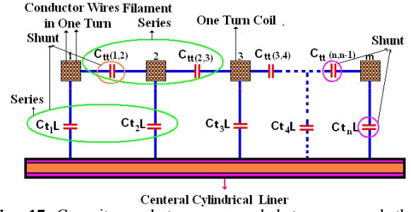
Fig. 17 Capacitance between wounded turns around the central liner.
