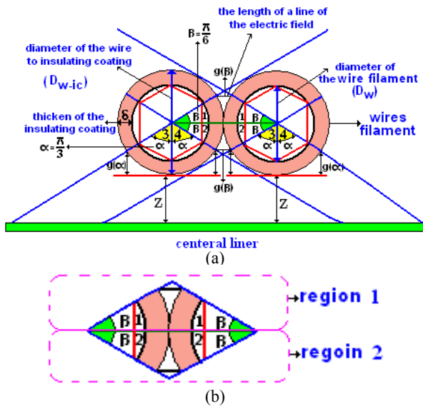
Fig. 8 View of the path g(\beta) of electric field lines E under angle \beta between two adjacent CWF in OTC of the generator [8]. a) View of g(\beta) path of electrical field lines under \beta angle. b) Two trapezium-shape regions 1 and 2 in ELBC.
