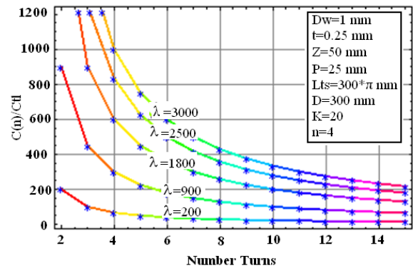
Fig. 20 Ratio of total capacitance of nTC of the generator to turn-liner capacitance C(n)/C_{tl} for different values of \lambda .
