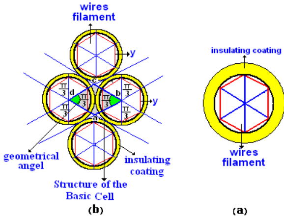
Fig. 7 An abcd equilateral lozenge-shape basic cell for calculating filament-filament capacitance [8]. a) Vespiary regular hexagon (VHR) region. b) abcd basic cell.
