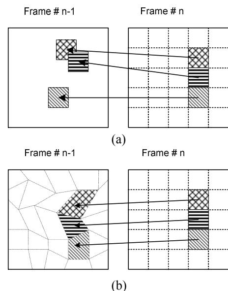
Fig. 1 Backward motion estimation: (a) Block-based, (b) Mesh-based.
