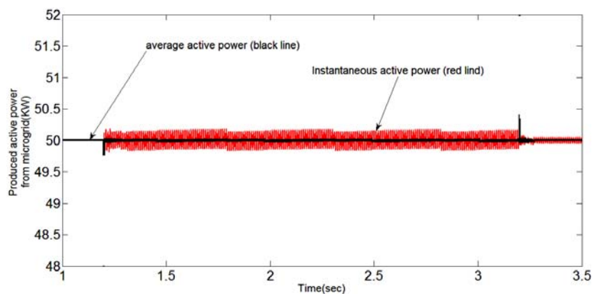
Fig. 18 average and instantaneous active power of microgrid
