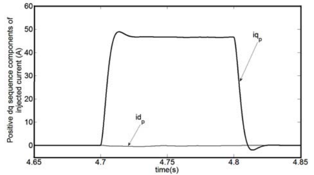
Fig. 22 Positive dq sequence components of injected currents by voltage source converter.
