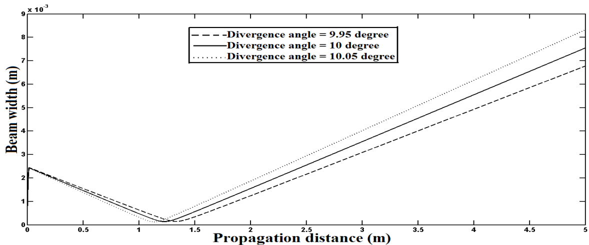
Fig. 2 Beam width variation versus propagation path length. Collimator-source separation ( L_0 ) is 9.352 mm.
