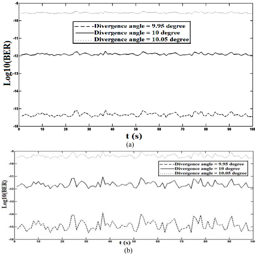
Fig. 7 BER for three different resulting divergence angles (1.04, 1.2, 1.36 mrad) due to source divergence angle variation, (a) the effect of beam deviation in the range of \pm 0.5 m (b) the effect of beam deviation in the range of \pm 1 m.
