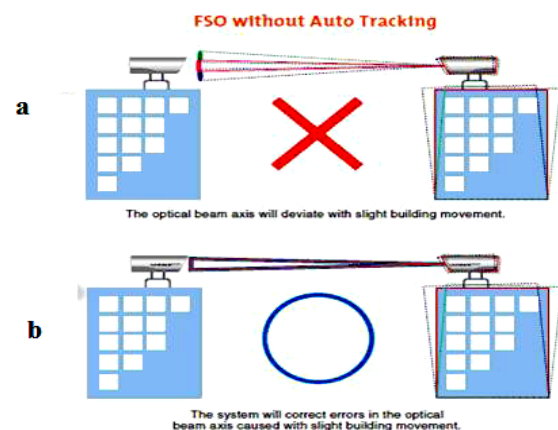
Fig. 5 Schematic representation of the auto-tracking subsystem effect, canon company.
