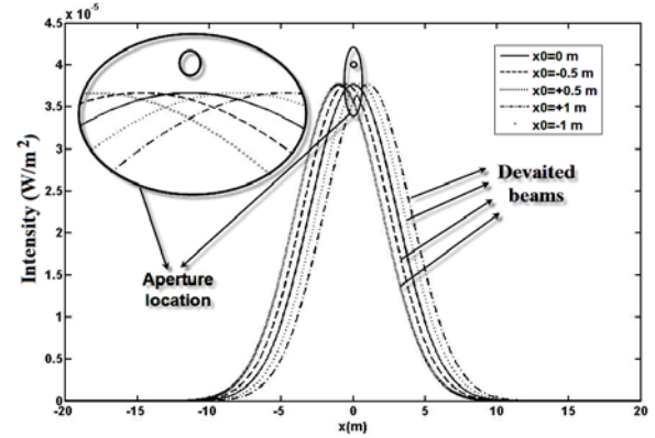
Fig. 6 Intensity distribution and receiver aperture situation for four different deviation values ( x_0 = \pm 0.5, \pm 1 m).
