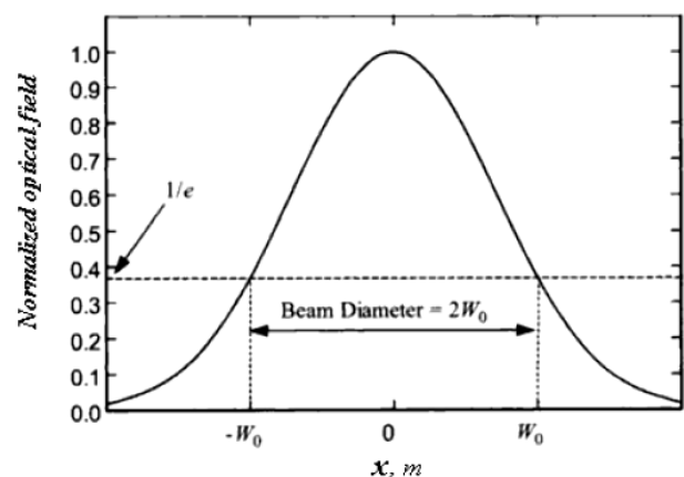
Fig. 3 Amplitude profile of a Gaussian beam wave [9].
