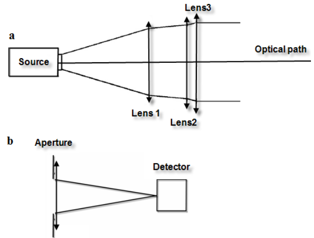
Fig. 1 (a) The layout of collimator A = 0.735 , B = 0.0098 , C = -72.416 , D = 0.399 (b) Schematic layout of optical receiver (lens, aperture and detector).
