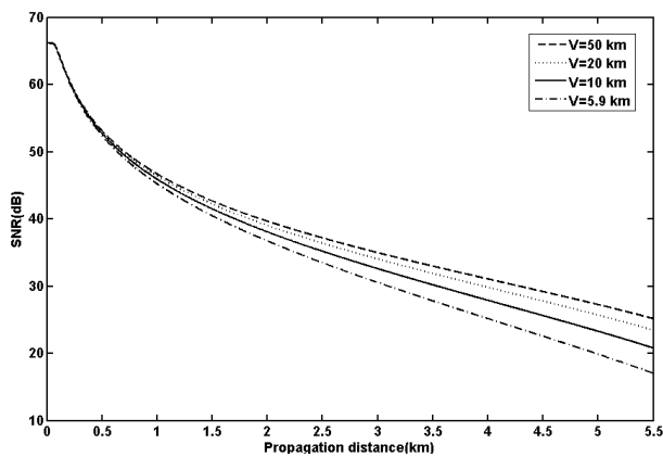
Fig. 9 SNR values versus propagation distance for four different visibility values (divergence angle = 1.2 mrad).
