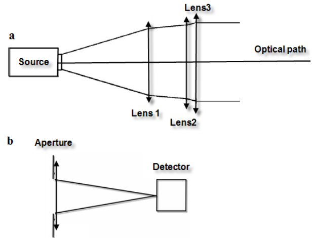
Fig. 1 (a) The layout of collimator A = 0.735 , B = 0.0098 , C = -72.416 , D = 0.399 (b) Schematic layout of optical receiver (lens, aperture and detector).
