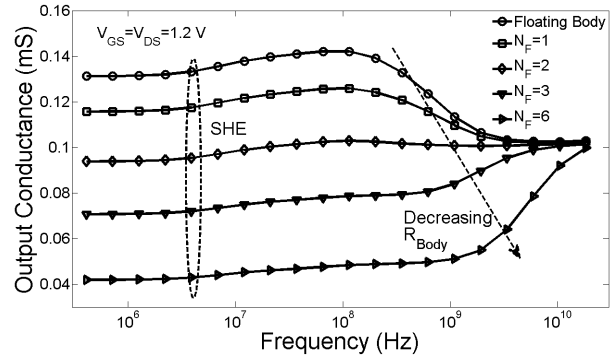
Fig. 4 Output Conductance vs. Frequency at V_{GS}=V_{DS}=1.2 V.
