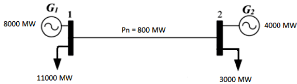
Fig. 2 Schematic of 2-bus test system.
