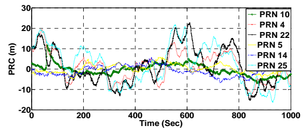
Fig. 8 DGPS PRC of PRN's 4, 22, 25, 14, 10 and 5.
