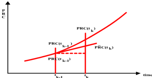
Fig. 2 Compensation PRC for time latency.
