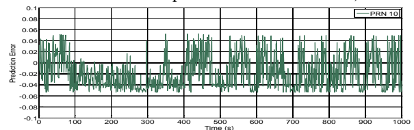
Fig. 10 One-step PRC prediction error of PRN 10
