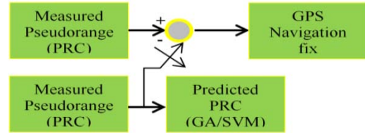
Fig.7. Architecture for predicting the PRC.
