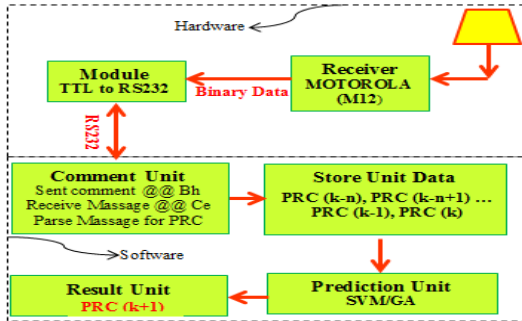
Fig. 5 Topology for PRC Prediction
