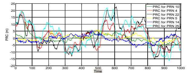
Fig. 8. DGPS PRC of PRN's 4, 22, 25, 14, 10 and 5
