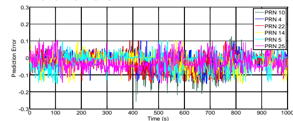
Fig. 15 10s ahead PRC prediction error of 6 satellites
