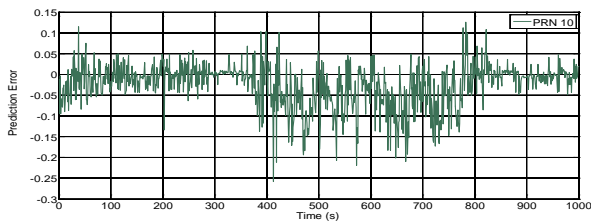
Fig. 11 10s ahead PRC prediction error of PRN 10
