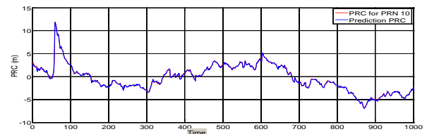
Fig. 9 DGPS PRC (PRN 10) prediction by GASVM
