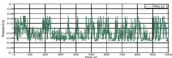
Fig. 13 One-step PRC prediction error of PRN 22
