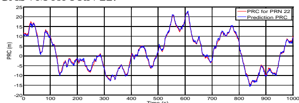
Fig. 12 DGPS PRC (PRN 22) prediction by GASVM
