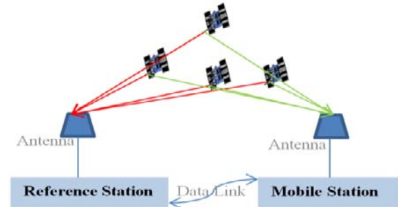
Fig. 1 Real time topology DGPS
