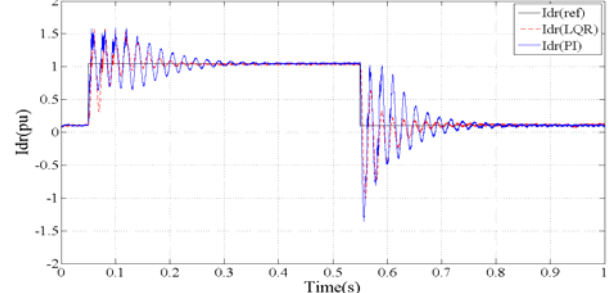
Fig. 10 D-axis component of Rotor current in fault condition.
