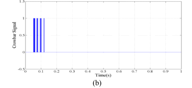
Fig. 9 The rotor currents and crowbar activation signal in fault condition using proposed LQR.
