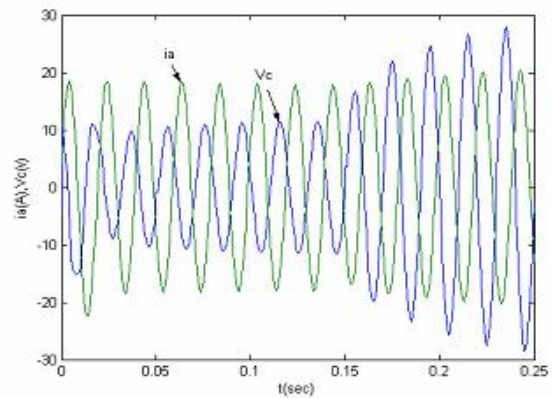
Fig. 9 Effect of increasing reactive power on injected voltage and line current
