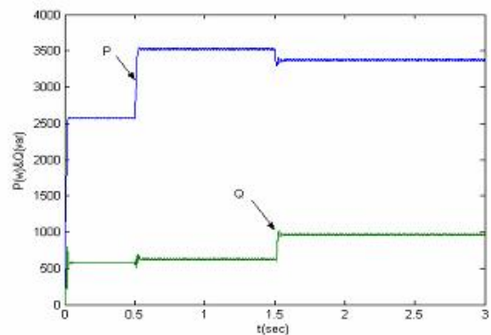
Fig. 5(b) Indirect control response to step changes
