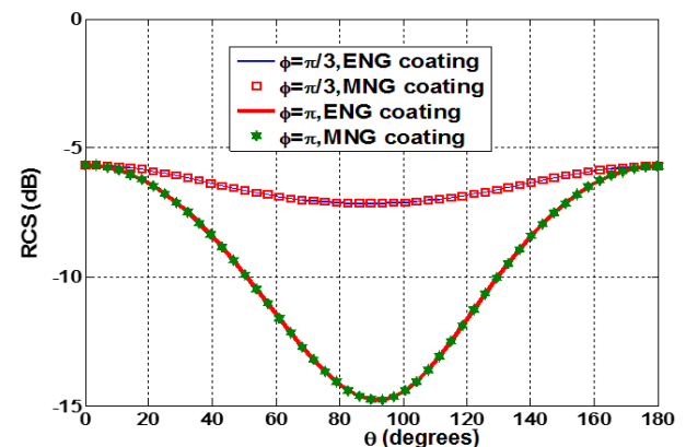
Fig. 3 The radar cross section of the conductor sphere coated with ENG materials and with MNG materials (the dual case) at frequency f = 7 GHz in the half planes \phi = \pi/3 and \pi versus different angles of observation \theta .
