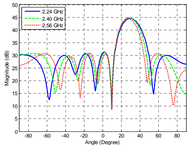
Fig. 5 Beamformer response in the lower passband.
