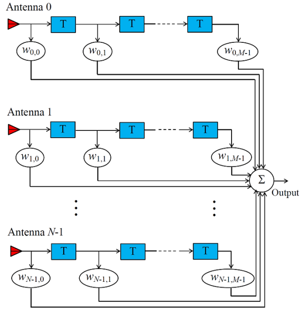
Fig. 1 General structure of a wideband TDL array antenna.
