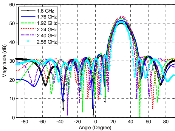
Fig. 2 Beamformer response in the lower passband.
