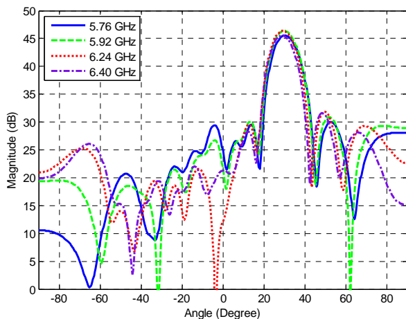
Fig. 7 Beamformer response in the upper passband.
