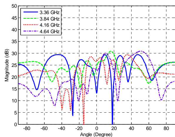
Fig. 6 Beamformer response in the stopband.
