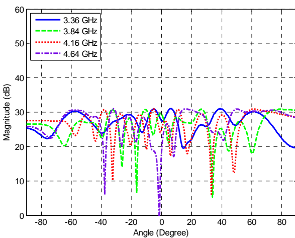
Fig. 3 Beamformer response in the stopband.
