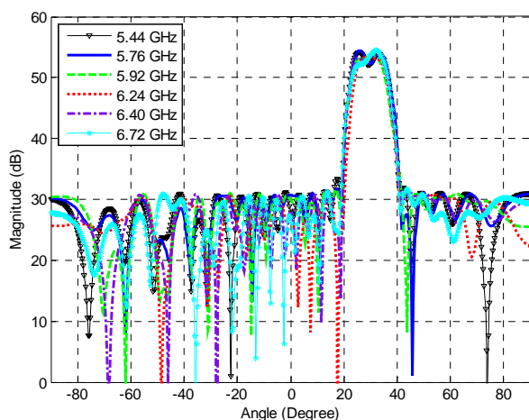
Fig. 4 Beamformer response in the upper passband.
