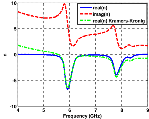
Fig. 4 The retrieved refractive index of the proposed structure.
