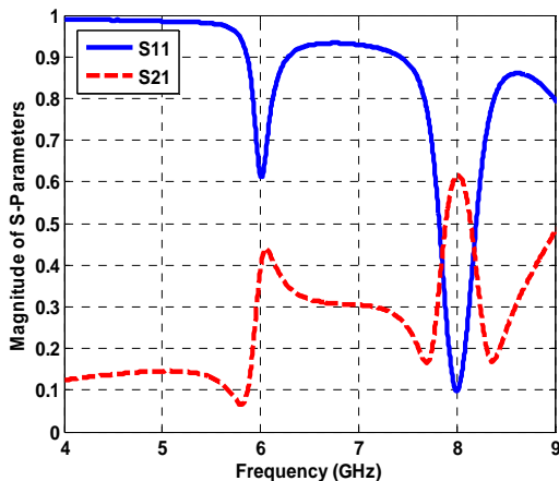
Fig. 3 Simulation results of the transmissions and reflection spectra.
