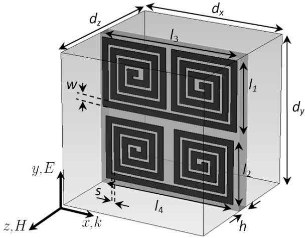
Fig. 1 Schematic diagram of the proposed dual-band magnetic structure unit cell. The geometric parameters of the unit cell are given by d_x = d_y = d_z = 2.5 mm, w = 0.1 mm, s = 0.05 mm, l_1 = 1.15 mm, l_2 = 1.05 mm, l_3 = 2.4 mm, l_4 = 2.3 mm, and h = 0.25 mm.
