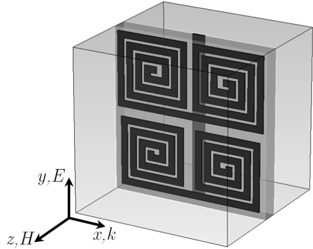
Fig. 2 Schematic diagram of the proposed dual-band magnetic structure unit cell. The geometric parameters of the unit cell are given by d_x = d_y = d_z = 2.5 mm, w = 0.1 mm, s = 0.05 mm, l_1 = 1.15 mm, l_2 = 1.05 mm, l_3 = 2.4 mm, l_4 = 2.3 mm, and h = 0.25 mm.
