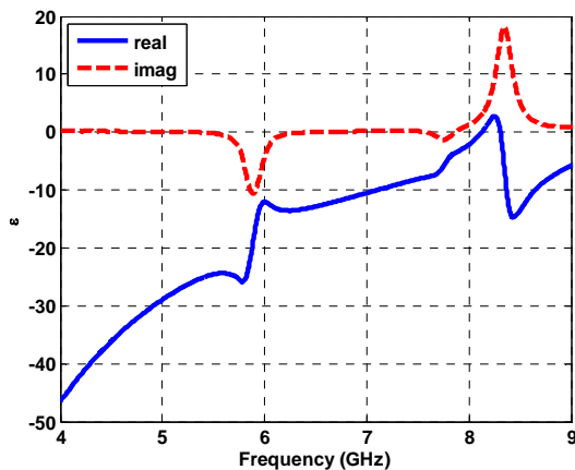
Fig. 5 The retrieved permittivity of the proposed structure.
