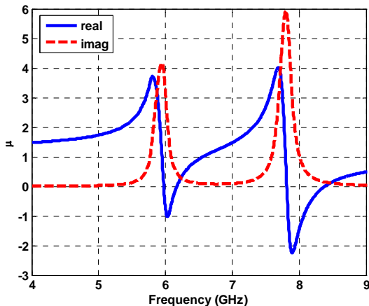
Fig. 6 The retrieved permeability of the proposed structure.
