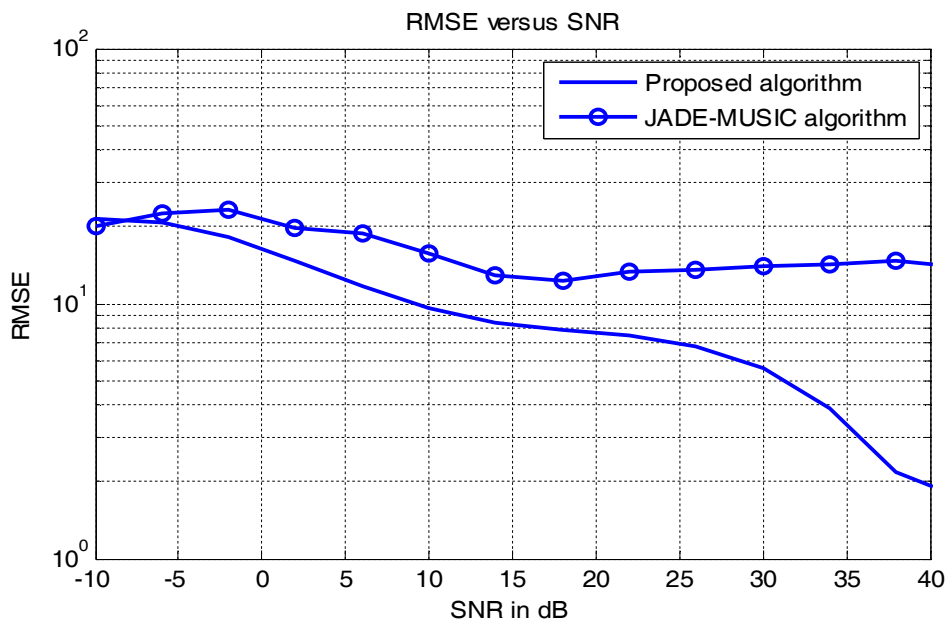
Figure 7. RMSE versus SNR for colored noise scenario
