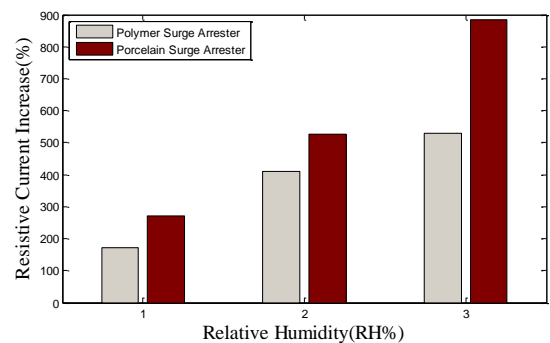
Fig. 5 Resistive leakage current increase measured in two Surge arresters in 14.4 kV applied voltage (x-axis: 1, corresponds to RH% range: (65-75%); 2, corresponds to RH% range: (75-85%) and 3, corresponds to RH% range: (85-95%))
