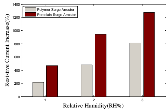
Fig. 3 Resistive leakage current increase measured in two Surge arresters in 11.5 kV applied voltage (x-axis: 1, corresponds to RH% range: (65-75%); 2, corresponds to RH% range: (75-85%) and 3, corresponds to RH% range: (85-95%))
