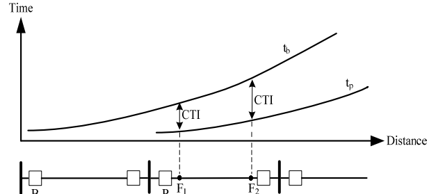
Fig. 1 Selectivity illustration for DOCRs.
