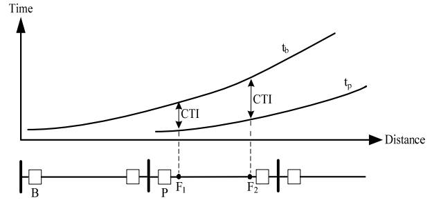
Fig. 1 Selectivity illustration for overcurrent relays.
