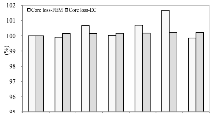
Fig. 8 Core loss under unbalanced voltages.
