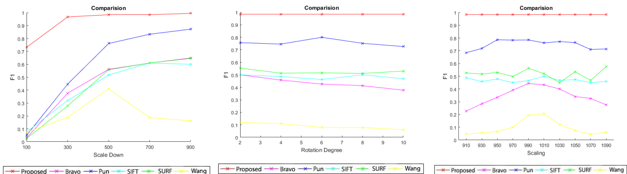
Fig. 4 Illustrating F1 in scale down, scaling, and rotation.
