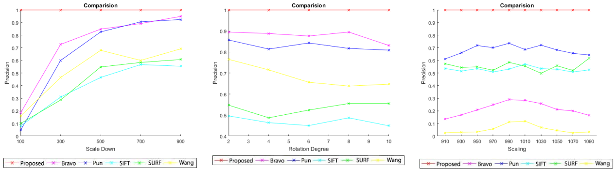
Fig. 5 Illustrating precision in scale down, scaling, and rotation.
