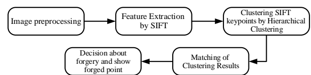
Fig. 1 Diagram of the proposed algorithm.
