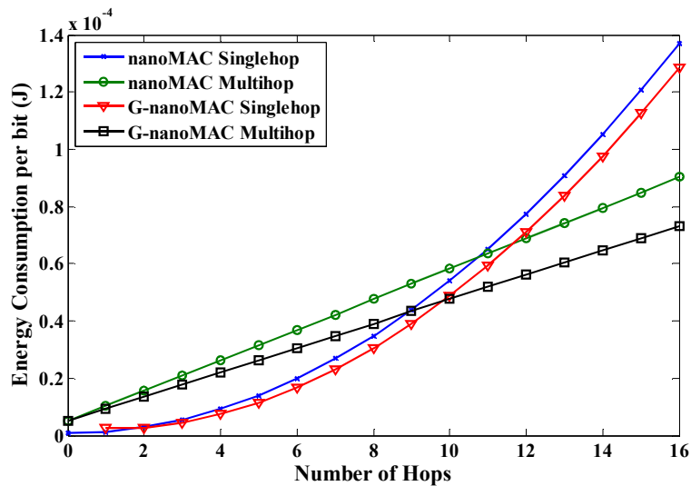
Figure 7 Energy consumption vs number of hops
