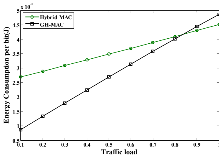
Figure 9 Energy consumption per bit vs traffic load
