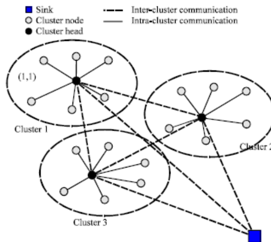
Figure 1 Overview of intra and inter cluster domain of WSN
