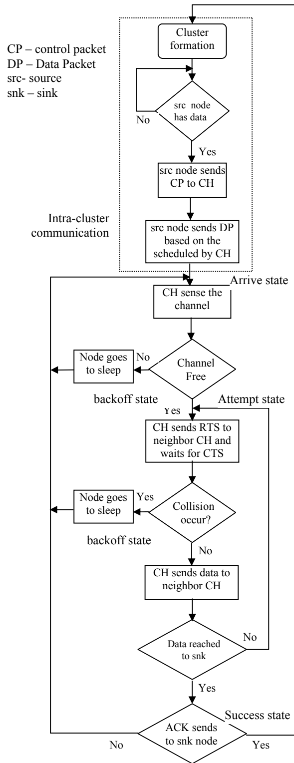
Figure 3 system model for Hybrid-MAC
