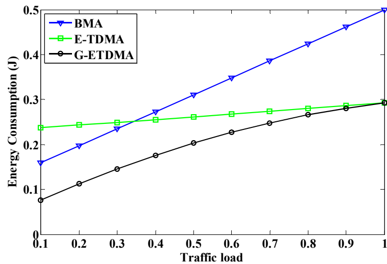
Figure 4 Average Energy Consumption vs traffic load (N=20 and k=5)
