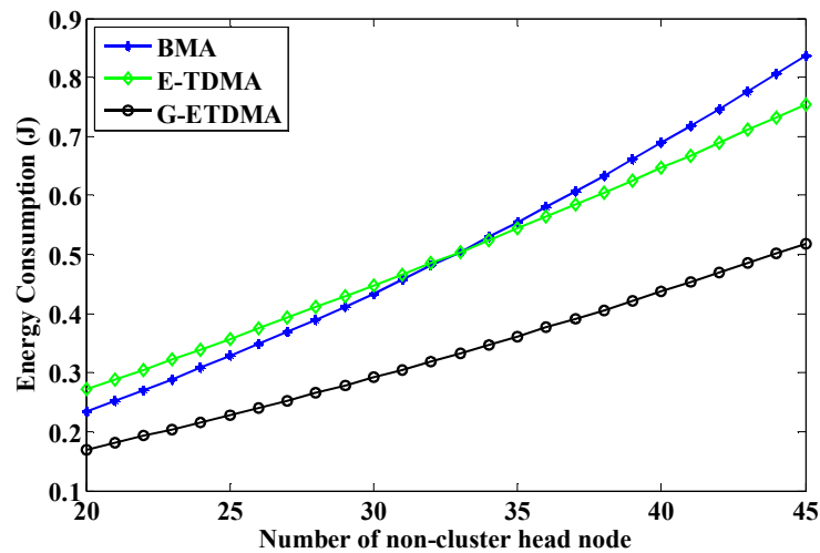
Figure 5 Average total cluster energy consumption vs. N ( k = 5 and traffic load is 0.4)
