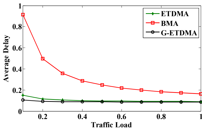
Figure 6 Average delay vs Traffic load
