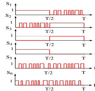
Fig. 3 Switching pulses of the proposed inverter.
