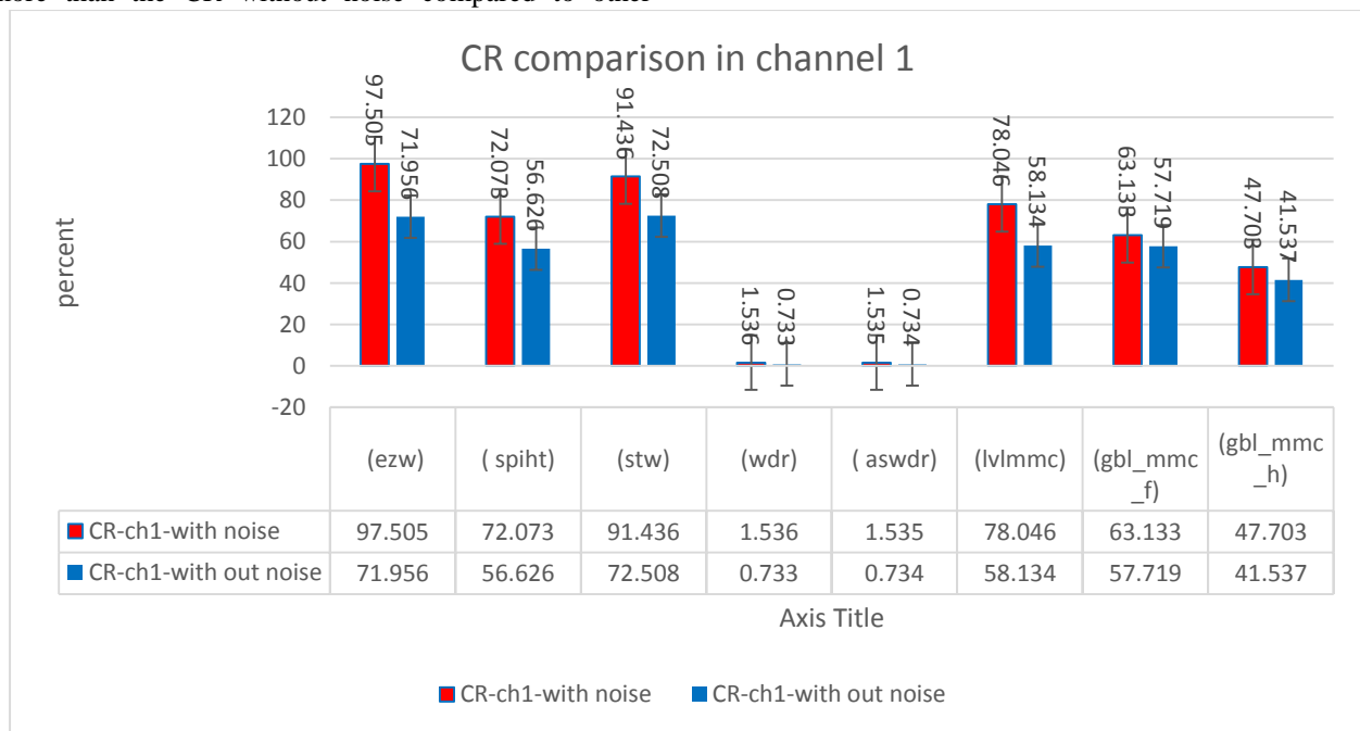
Fig. 4 CR values in different compression methods with and without noise channel 1
