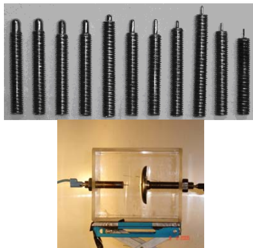
Fig. 3 Hemispherically-capped steel rod electrodes and test object.
