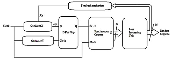
Fig 5. BFD PRNG architecture using feedback mechanism.
