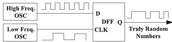
Fig 2. Ring oscillator-based TRNG.
