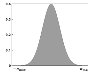
Fig 7. Gaussian probability distribution function.
