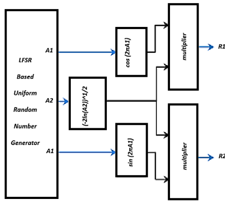
Fig 8. Conventional Box-Muller based GRNGs.
