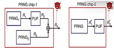
Fig 9. ML resistant PRNG.
