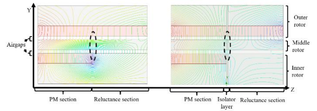
Fig 3. Flux line distributions between PM and Reluctance sections of the proposed model (left) without an isolation layer and (right) with an isolation layer.
