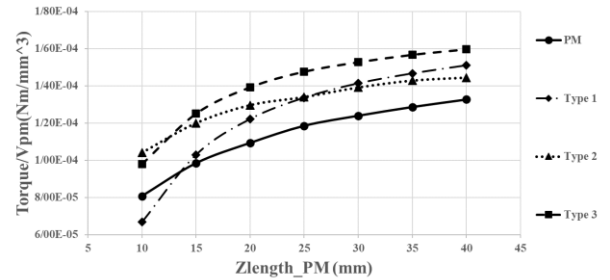
Fig 23. Torque-to-magnet volume ratio of different MG configurations in different PM MG lengths.
