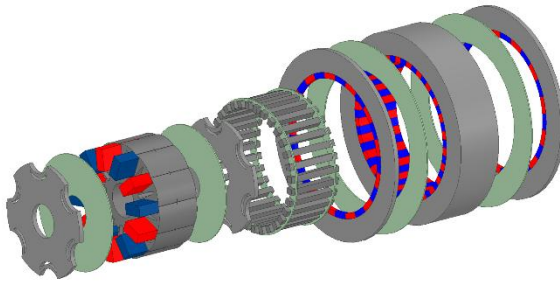
Fig 26. Exploded view of the proposed model.
