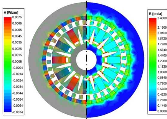
Fig 14. The distribution of flux density (right) and magnetic potential lines (left) in the PM rotor structure.
