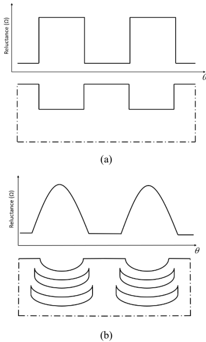
Fig 7. Reluctance comparison of (a) the simple teeth and slot model and (b) the proposed model.
