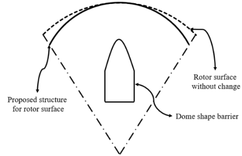
Fig 5. The decentralized and dome-shaped barrier.
