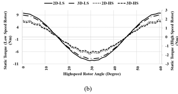
Fig 17. (a) Dynamic torque and (b) Static torque results of the reluctance rotor MG design regarding the high-speed rotor angle.
