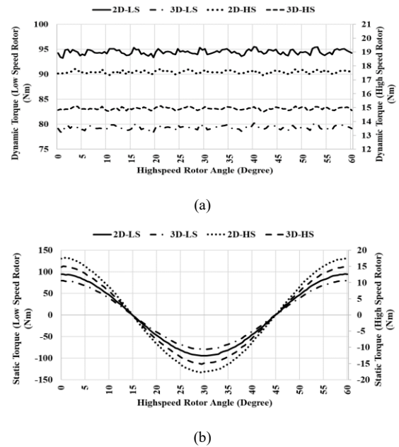
Fig 12. (a): Dynamic torque result and (b): Static torque result of the PM rotor design regarding the high-speed rotor angle.
