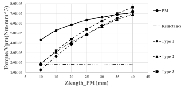
Fig 24. Torque-to-total magnet volume (inner and outer rotors) ratio of different MG configurations in different PM MG lengths.
