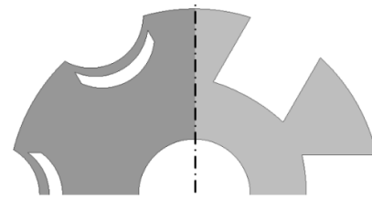
Fig 16. The optimal (right) initial and (left) proposed reluctance design.
