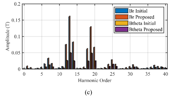
Fig 18. Magnetic flux density in the inner air gap proposed reluctance design (a) radial component, (b) tangential component, and (c) FFT analysis results.
