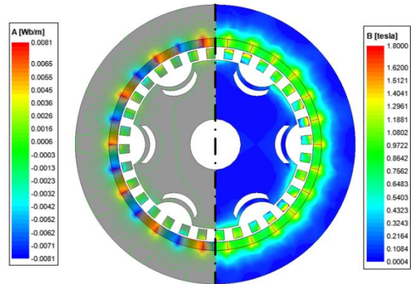
Fig 19. The distribution of flux density (right) and magnetic potential lines (left) in a reluctance rotor design.
