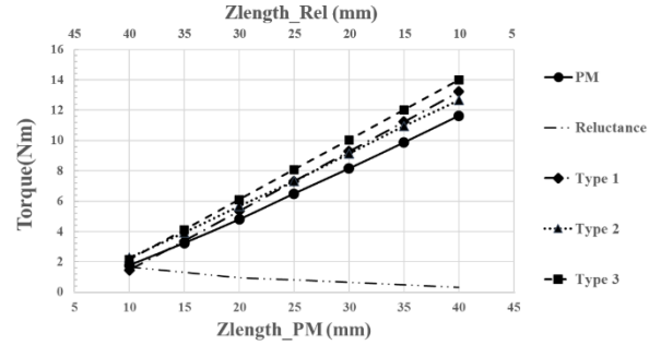
Fig 22. Torque of different MG configurations in different PM MG lengths.
