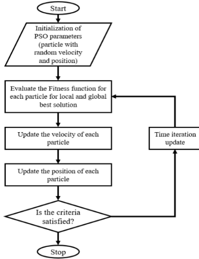
Fig 9. PSO flowchart.
