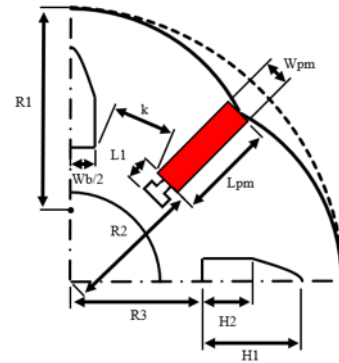
Fig 6. Design parameters of the PM rotor.
