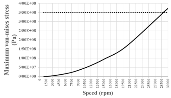
Fig 27. The maximum von Mises stress of the inner core based on the speed.
