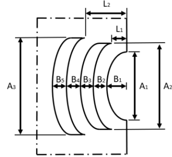
Fig 8. Design parameters of the reluctance rotor.
