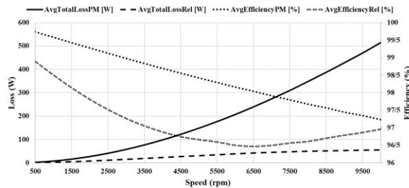
Fig 20. Loss and efficiency of proposed designs at different speeds.
