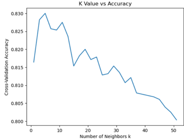
Fig 18. Accuracy versus k curve for the kNN algorithm.
