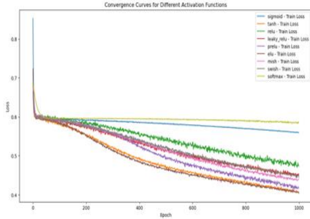
Fig 20. Comparison of the network's loss with different activation functions.
