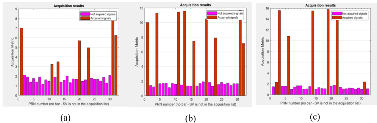
Fig 4. Acquisition level of the signal: (a) authentic, (b) spoofed 6sec, and (c) spoofed 4sec.
