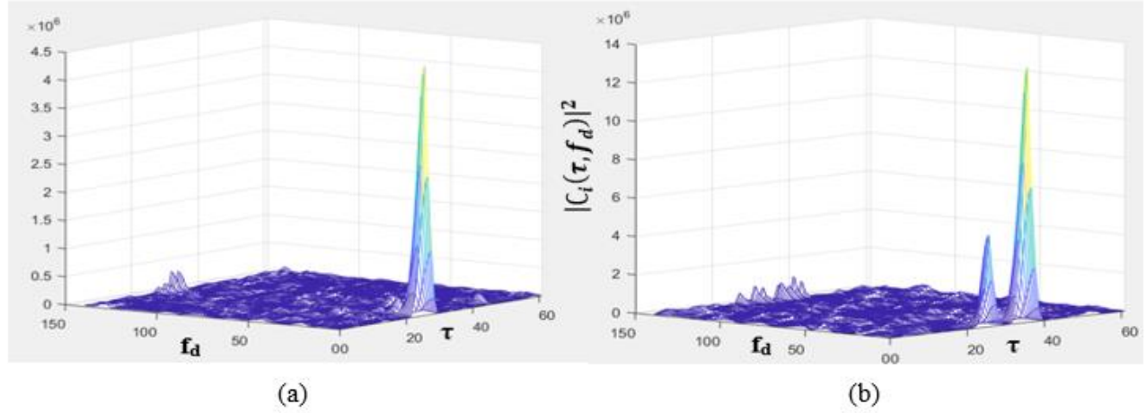
Fig 2. Evaluation of the CAF over the delay/Doppler frequency grid with C/N_0=25\text{--}30 dB-Hz and a delay of less than 0.75 chips for: (a) the hypothesis H_0 , and (b) the hypothesis H_1 .
