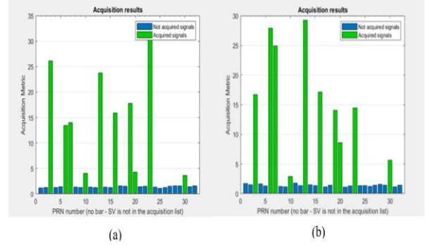
Fig 6. Acquisition level of the TEXBAT data signal: (a) authentic, and (b) spoofed.
