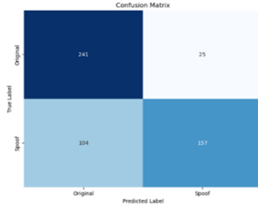
Fig 14. Confusion matrix of the MLP neural network in the proposed method on 6Sec dataset.
