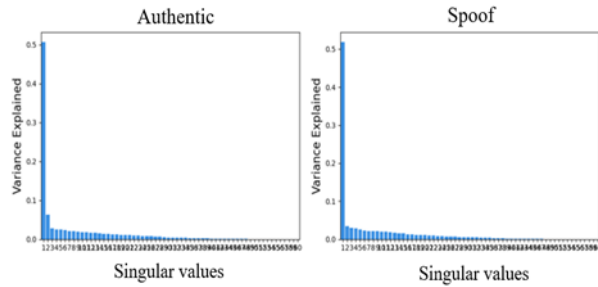
Fig 9. Explained variance for the 6sec dataset.
