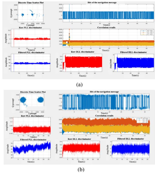
Fig 5. Tracking results for the spoofed signal: (a) 4 seconds, and (b) 6 seconds.
