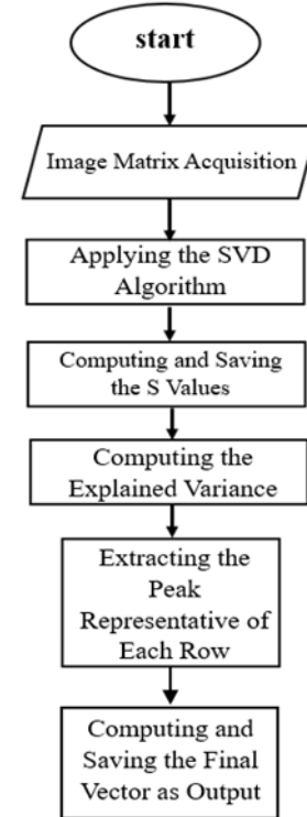
Fig 8. Diagram of the SVD_VAR algorithm.
