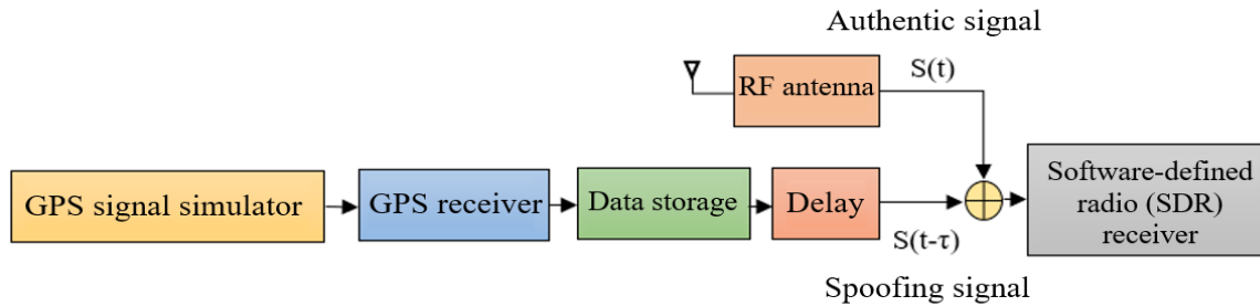
Fig 3. Block diagram of delayed spoofing signal generation.
