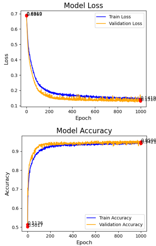
Fig 17. Training and validation accuracy and loss for the TEXBAT ds7 dataset generated using the proposed method on the MLP neural network.
