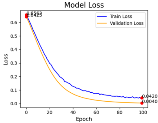
Fig 16. Training and validation accuracy and loss for the TEXBAT ds4 dataset (dimensions 1 \times 2 ) generated using the proposed method on the MLP neural network.
