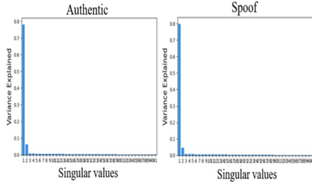
Fig 11. Explained variance for the TEXTBAT ds4 dataset.
