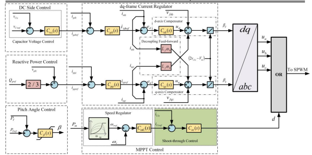
Fig 5. The comprehensive Schematic representation of a grid-connected qZSI control block in Wind turbine-based PMSG.
