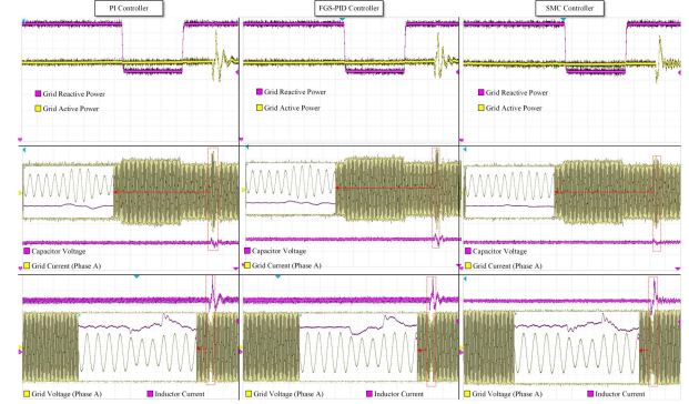
Fig 12. Obtained experimental HIL results of the 3 MW WECS based three phase qZSI using the conventional PI and FGS-PID and the SMC controllers, where the measured grid reactive power ( Q_g ) and active power ( P_g ), the grid current ( i_{ga} ) and capacitor voltage ( v_{C1z} ) with zoom for some switching cycles, the inductor current ( i_{L1z} ) and grid voltage ( v_{ga} ) are shown from top to bottom.
