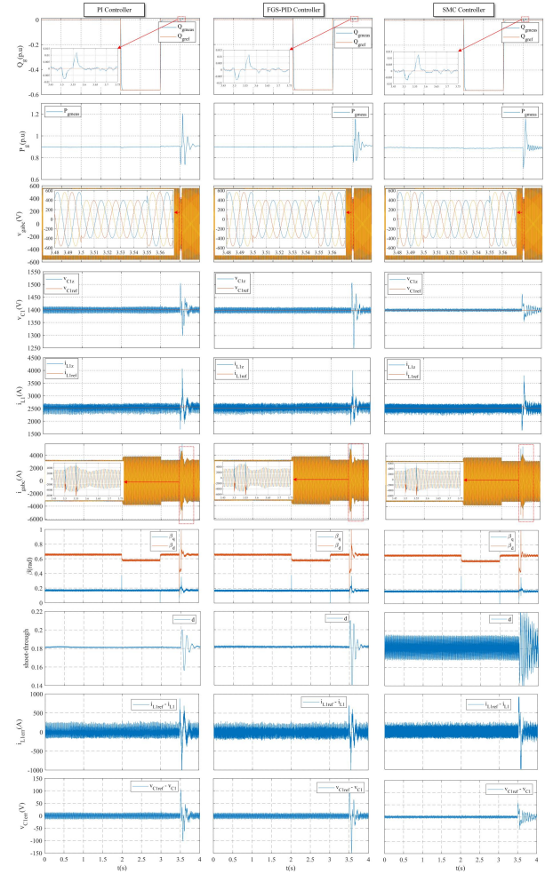
Fig 10. Obtained short simulation results of the 3 MW WECS based three phase qZSI using the conventional PI and FGS-PID and the SMC controllers, where the measured grid reactive power ( Q_g ) and active power ( P_g ), the grid voltages ( v_{gabc} ), the inductor current ( i_{L1z} ), the capacitor voltage ( v_{C1z} ), grid currents ( i_{gabc} ), the modulation indices ( \beta_{d,q} ), shoot through duty cycle ( d ), the inductor current error signal ( i_{L1err} ) and the capacitor voltage error signal ( v_{C1err} ) are shown from top to bottom.
