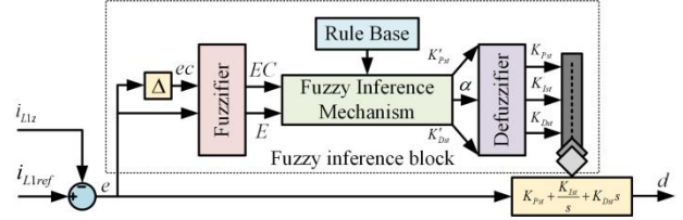
Fig 6. Structure diagram of inductor current control based on fuzzy inference.
