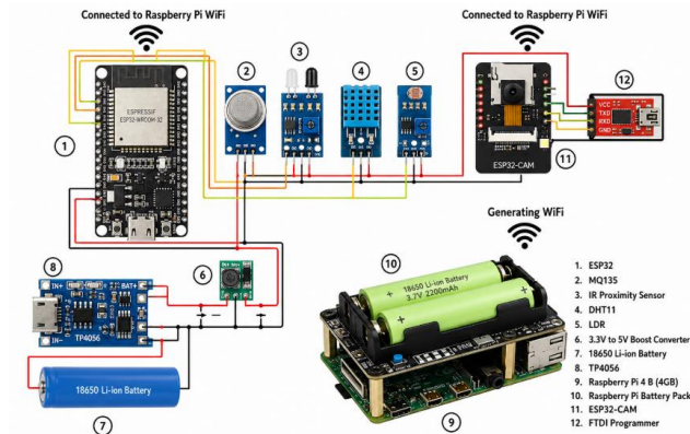
Fig 6. Hardware circuit implementation corresponding to the architecture.
