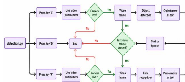
Fig 3. Working procedure for face recognition.
