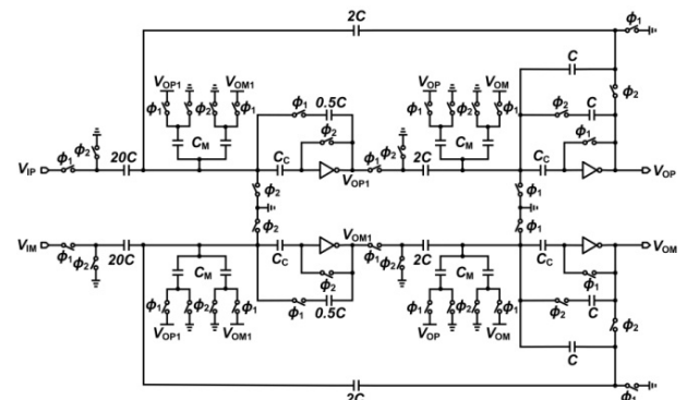
Fig. 8 Differential inverter-based SC low pass implementation.
