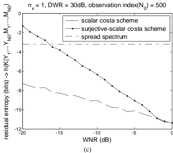
Fig. 7 Residual entropy comparison between SSCS and SCS.
